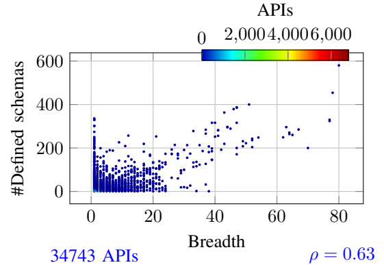
Fig. 6: Density scatter plots between #Paths and Breadth (X axis) and data model size metrics (Y axis). Each dot corresponds to one or more APIs having the same metric values.
