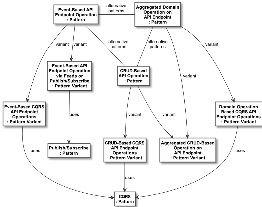
Fig. 2. Overview of the patterns and their relations
