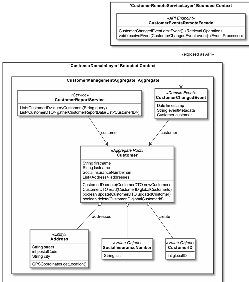
Fig. 6. Event-Based API Endpoint Operations for a Customer Changed Event
