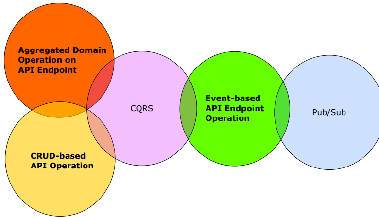
Fig. 1. High-level overview of the patterns
